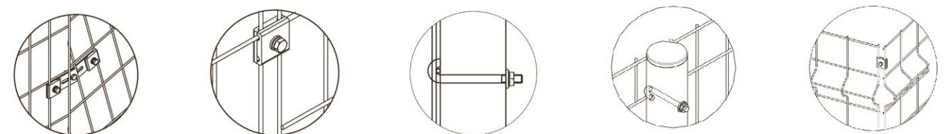
Wire mesh connection styles
